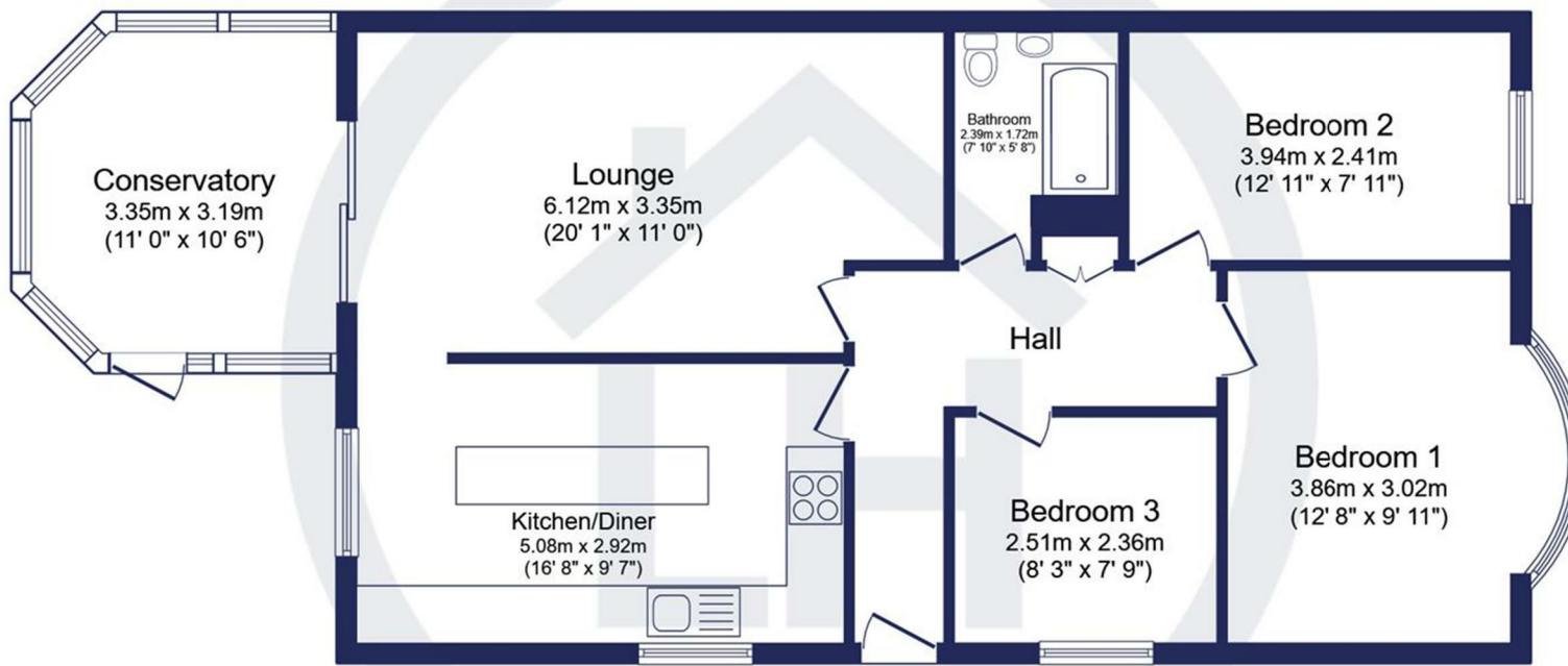
Ground Floor Floor area 88.6 sq.m. (954 sq.ft.)
